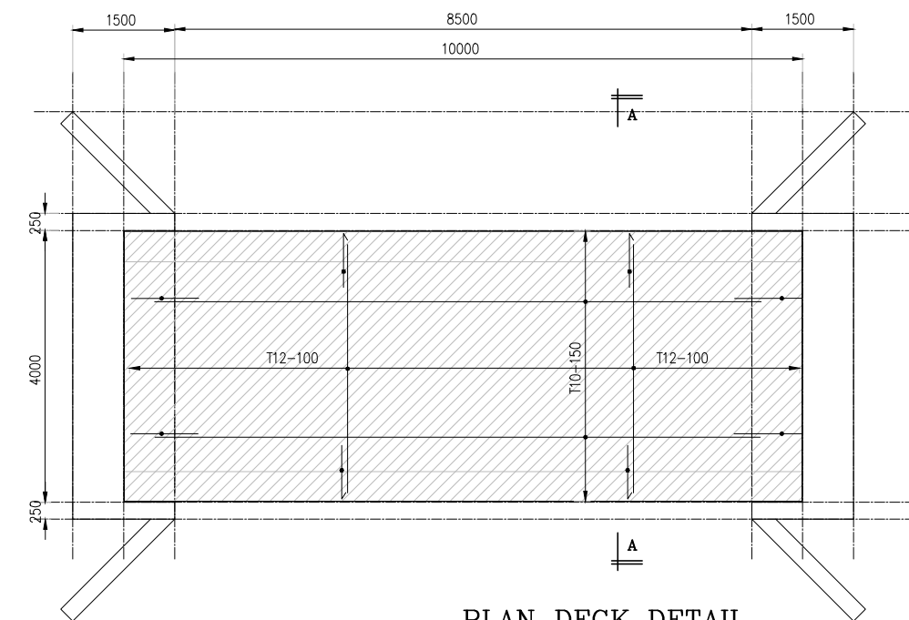
PLAN DECK DETAIL
