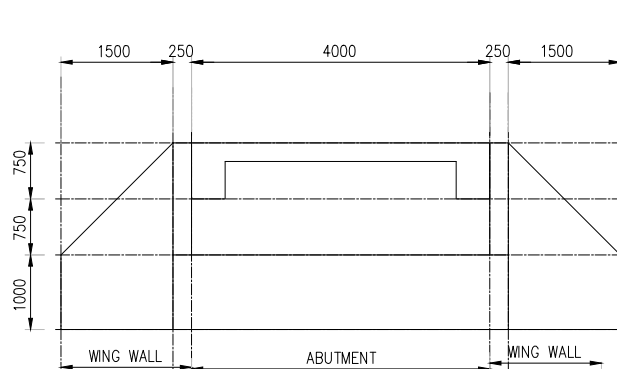
SECTION 1-1
