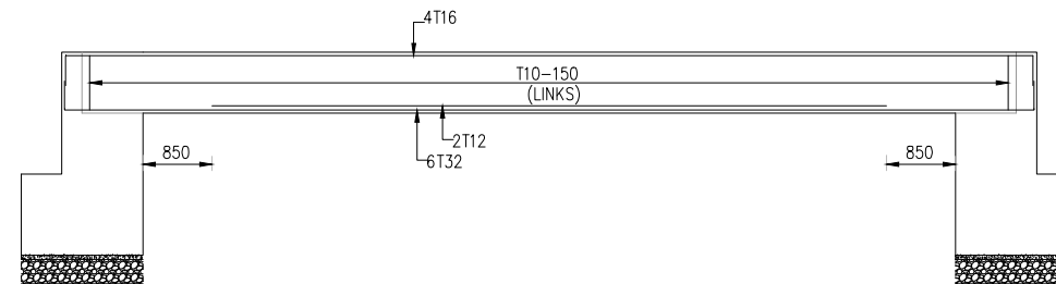
RC BEAM (450 X 750)
