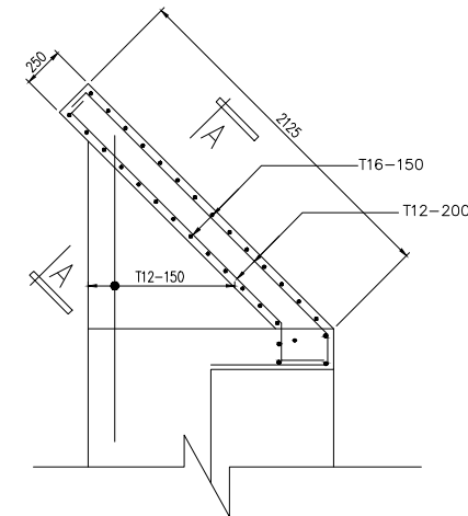
TYPICAL WING WALL DETAIL
