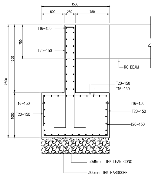
ABUTMENT DETAIL
